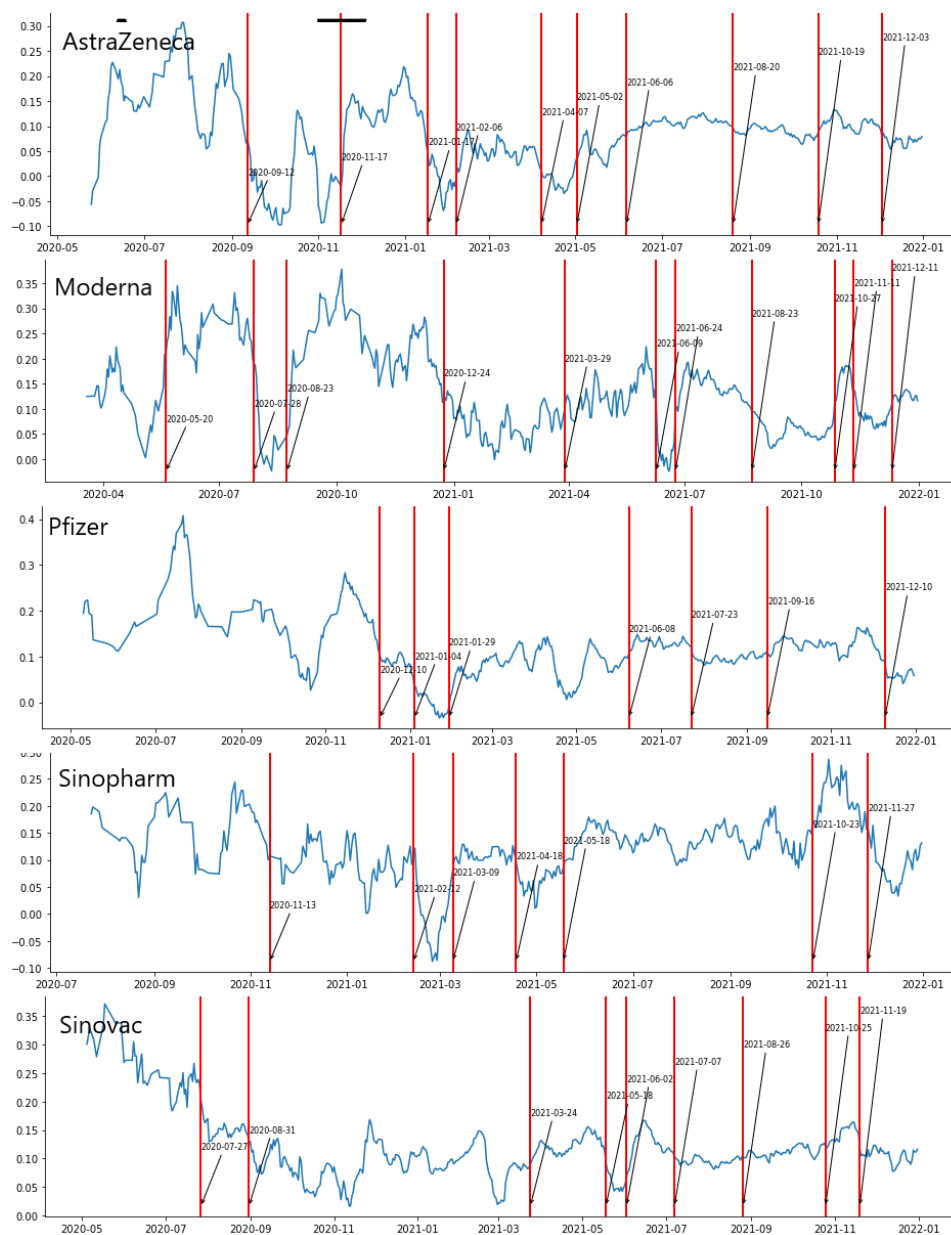
Figure 2. Change points of sentiment scores across time
